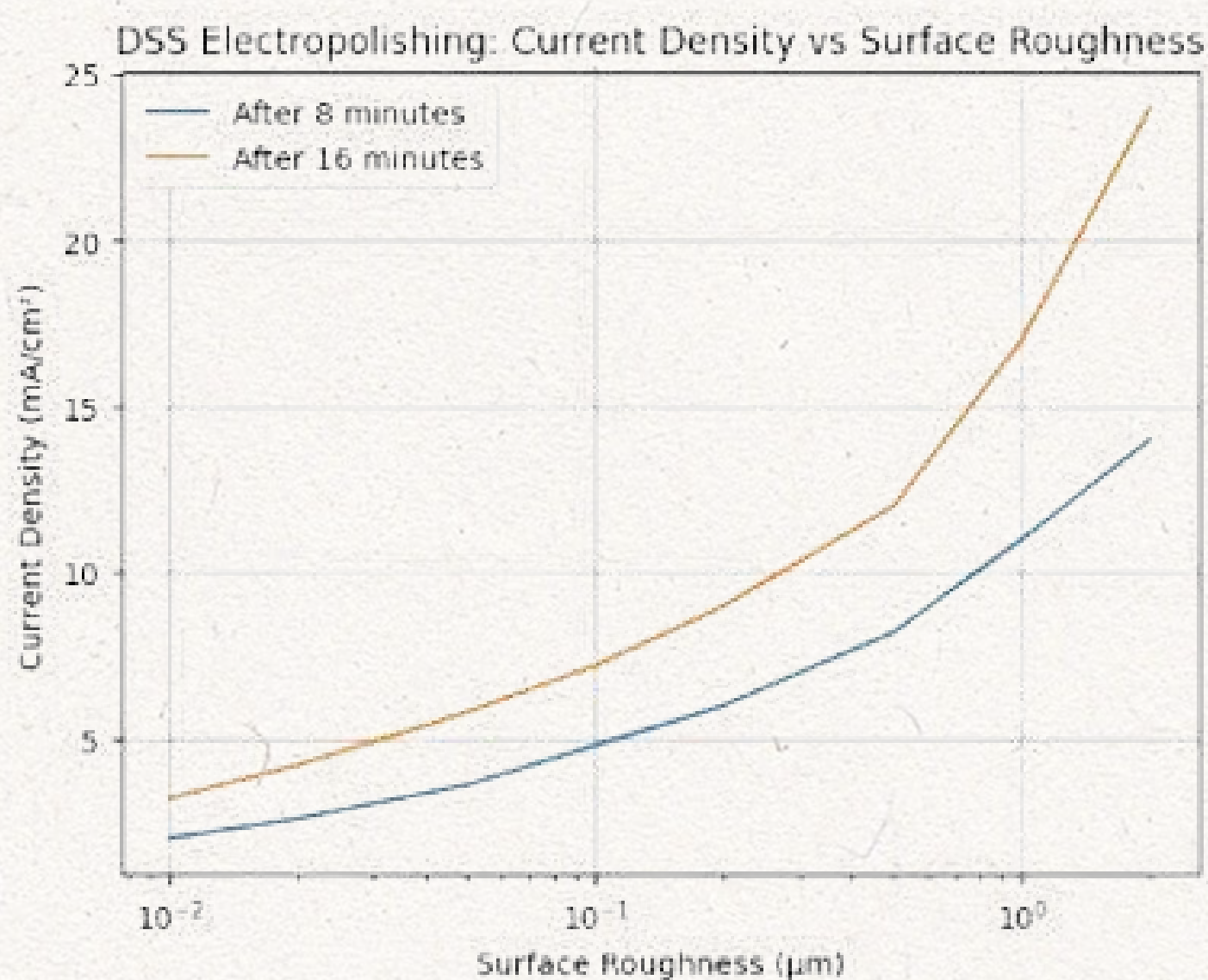
Fig 5. Effect of surface roughness on current density during electropolishing of duplex stainless steel. At a surface roughness of approximately 0.02 μm, stable current density behaviour is observed, indicating effective surface levelling within the limiting current region.
